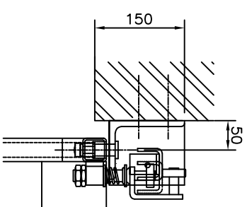
ENLARGED HEAD DETAIL
