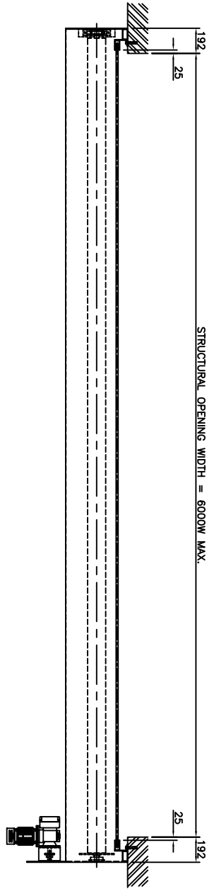
GALVANISED STEEL GRILLE (CHAIN DRIVE MOTOR) – UP TO 6000W x UP TO 2500H
