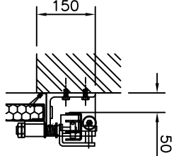
ENLARGED HEAD DETAIL
