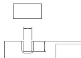
DETAIL 'Z' BOTTOM TRACK DETAIL
