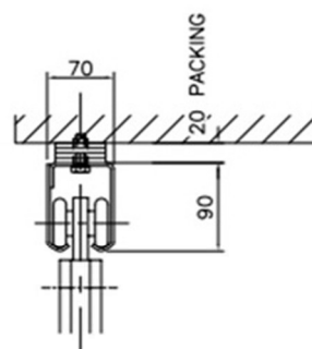
90mm TOP TRACK DETAIL
